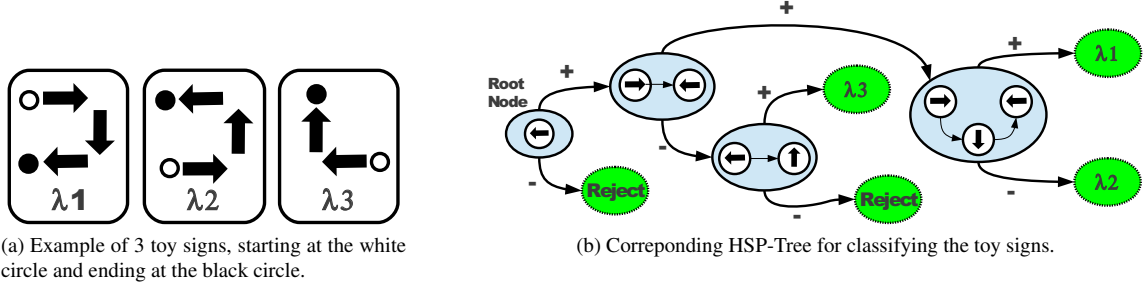
Figure 2: Illustration of how the HSP-Tree combines sequential patterns of three toy signs (a) to form a multi-class classifier (b). Non-leaf nodes are shown in blue with its associated SIP. For clarity, the SIP temporal intervals are not shown. Leaf nodes are shown in green. The link types are denoted by the + , - signs. Importantly, the HSP-Tree allows two SPs with any common subsequences (which may be in the middle of both SPs) to be merged. This type of sharing would not be possible with the SP-Tree method.
