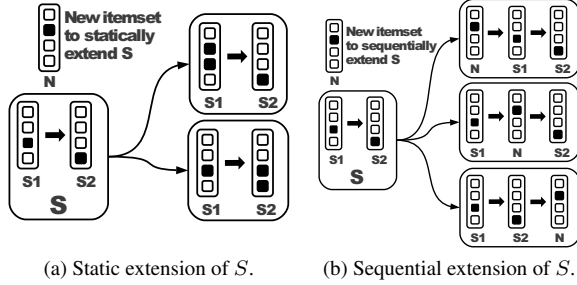
Figure 3: Methods for extending a SP or SIP.
