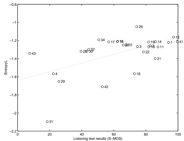
Fig. 4: The values of the EntropyL metric plotted against the S-MOS results from the listening test for the centre listening position. The numbers on the graph show the different DUTs used in the listening tests (see [5]).
