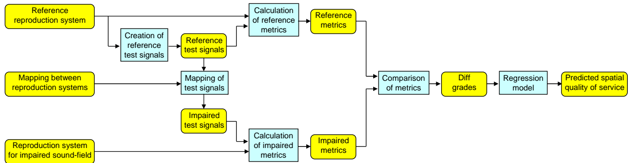
Fig. 1: Flow diagram showing the processes in the QESTRAL model, including the use of the test signals. The yellow rounded boxes show data, while the blue rectangular boxes show processes.
