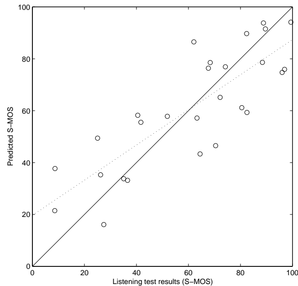
Fig. 3: Results of the cross validation of the regression model calibrated for the right listening position.
