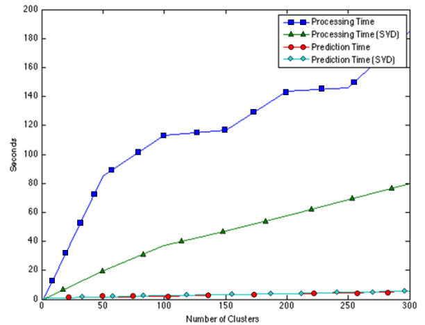
Fig. 14: Processing time for the clustering process
