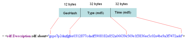
Fig. 11: Naming and ID construction
