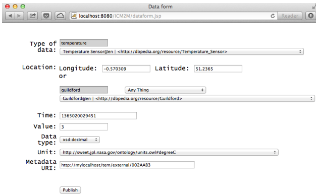
Fig. 6: The semantic stream annotation tool
